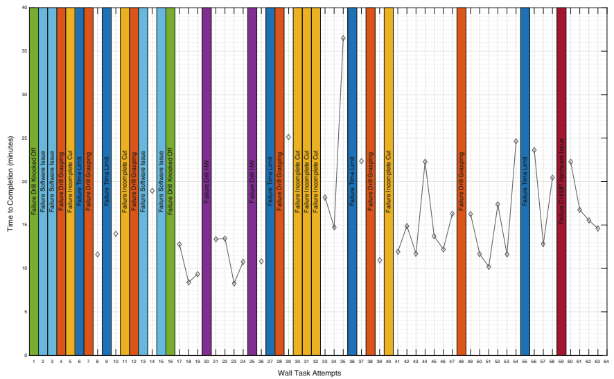
Fig. 8 Evolution of task time and success rate over time for the wall task. In early attempts, both software and process needed improvement to fix reliability due to overly aggressive drill grasping and cutting strategies. As development continued the success rate improved and execution times stabilized
