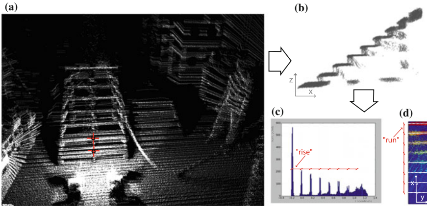
Fig. 5 Perception routine for “rise” and “run” estimation. a Operator inputs: clicks on 2 different steps. b LIDAR points in the region of interest around the stairs (lateral view). c Height histogram for points in the considered region of interest. d Top projection of the stairs points colored by step
