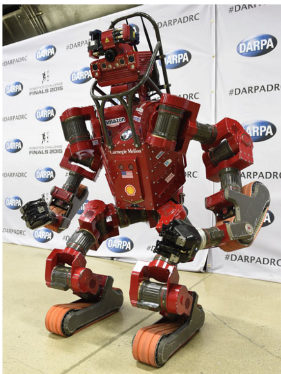
Fig. 1 CHIMP, the CMU highly intelligent mobile platform, designed and built at Carnegie Mellon's National Robotics Engineering Center
