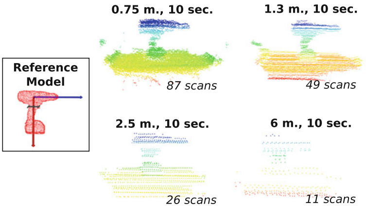
Fig. 11 Density of the point clouds captured for the drill at different distances (using a 10s accumulation buffer for the LIDAR scans)
